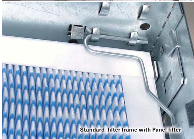
Panel filter (dusty air side)
