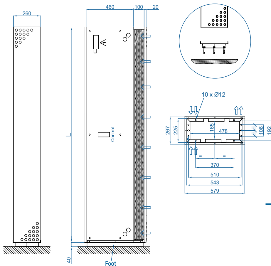
Vertical installation
