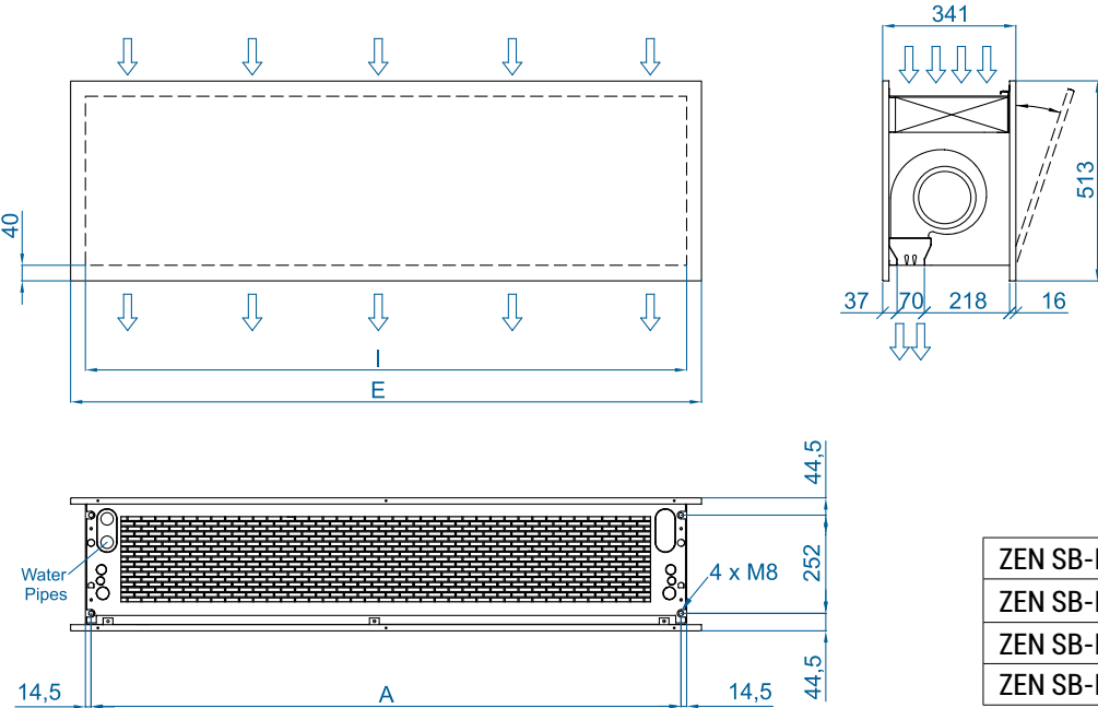
Horizontal installation
