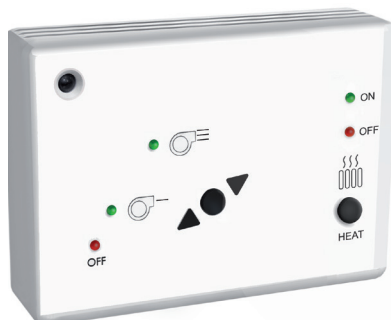
Controller for curtains with water battery
