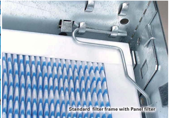
Panel filter (dusty air side)
