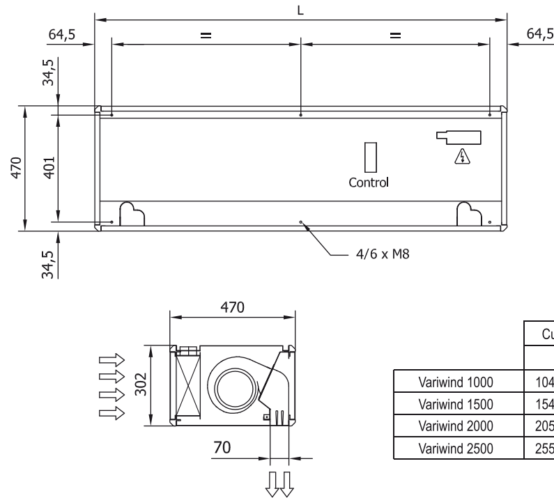
Variwind VP (With Profiles Construction)
